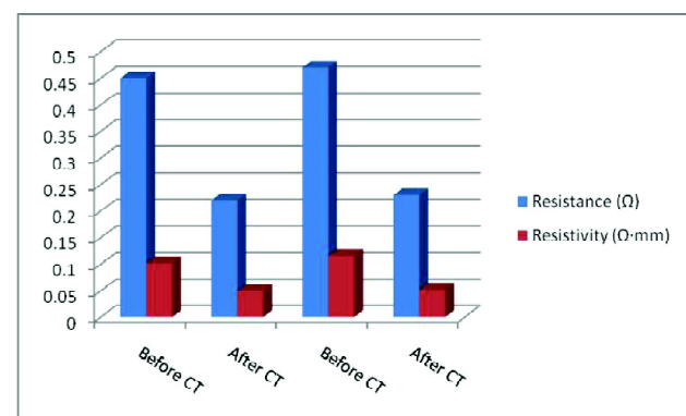
Fig. 6: Bar Chart of Resistance and Resistivity
